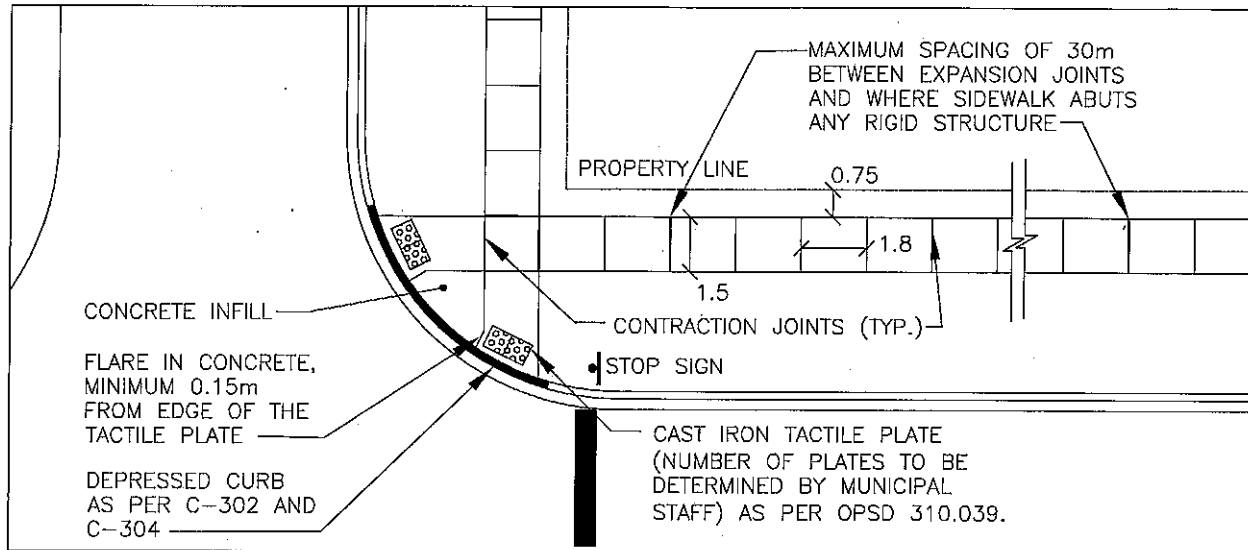
TYPICAL FLUSH CONTRACTION JOINT
