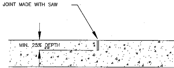
TYPICAL FLUSH CONTRACTION JOINT
